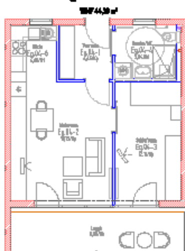
1 Pers.-Whg
